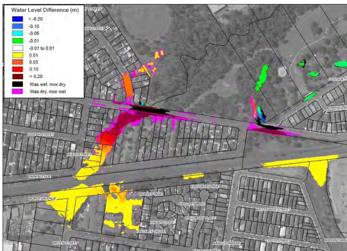
Plate 62 1% AEP flood level difference map for RM9 (elevated roadway only)
