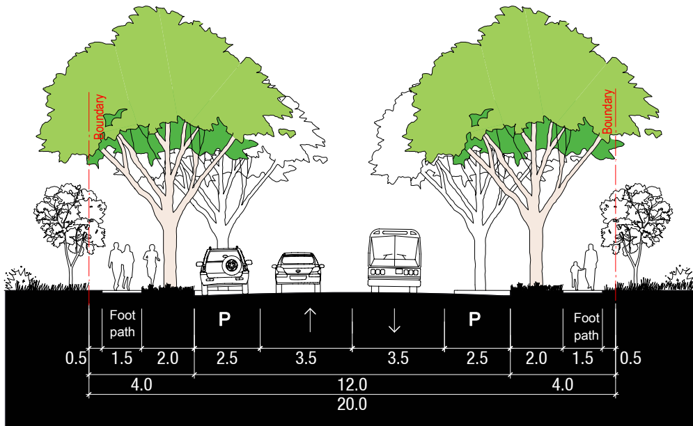
Collector Road (C1) with parking both sides
