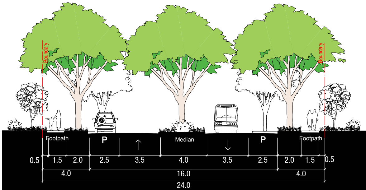
Collector Road with Median (C2) with parking both sides
