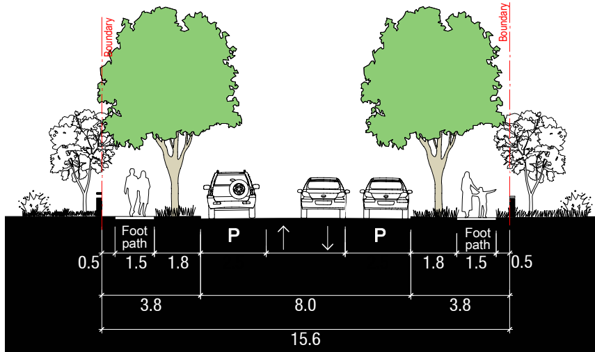
Minor Local Street (L1) with parking both sides
