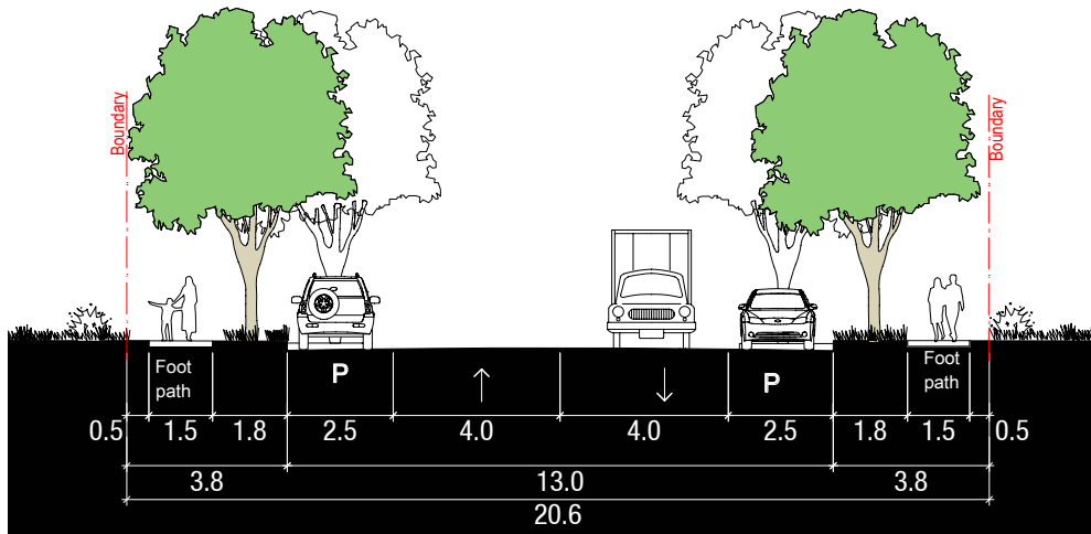
Employment Street (E1) with parking both sides
