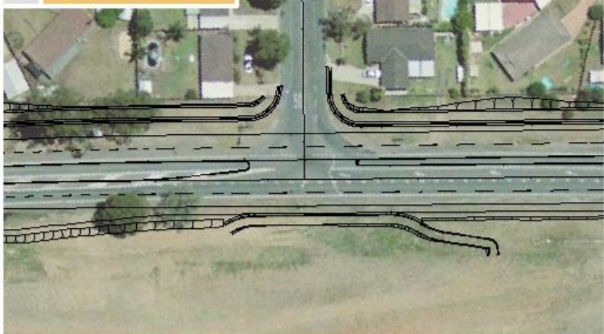
New signalled intersection at Bennett Road
