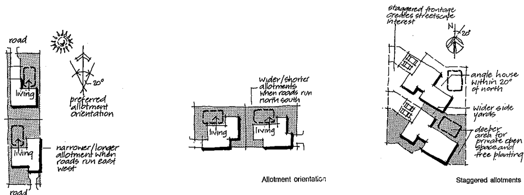
Figure - C11.2: Examples of Allotment Orientation
