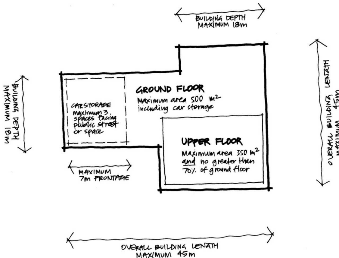
Figure D1.5: Maximum site coverage and building lengths for dwellings
