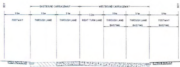
SECTION B HENRY STREET NTS
