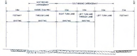
SECTION A EVANS STREET NTS
