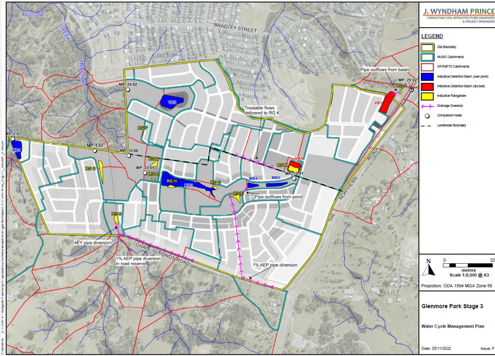
Figure E7.60 Indicative Water Cycle Management
