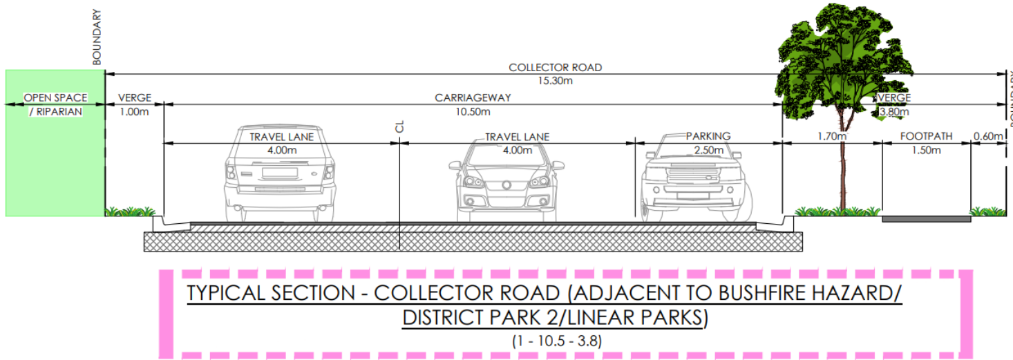
Figure E7.72 Collector Road (Adjacent to Bushfire Hazard / Passive -District Park 2 / Linear Parks
