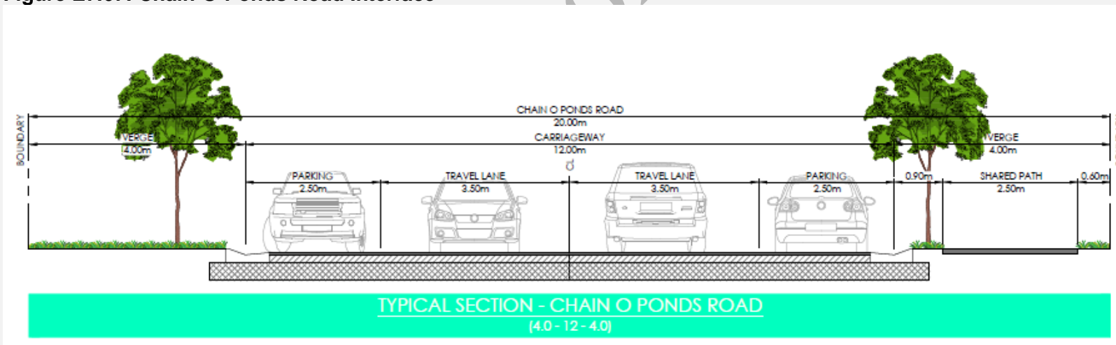
Figure E7.67: Chain-O-Ponds Road Interface
