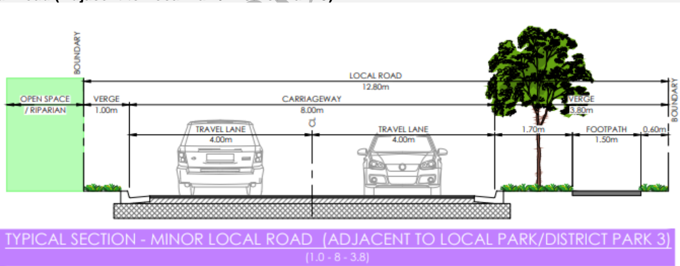
Figure E7.78-79 Minor Local Road (Adjacent to Local Park/ District Park 3)
