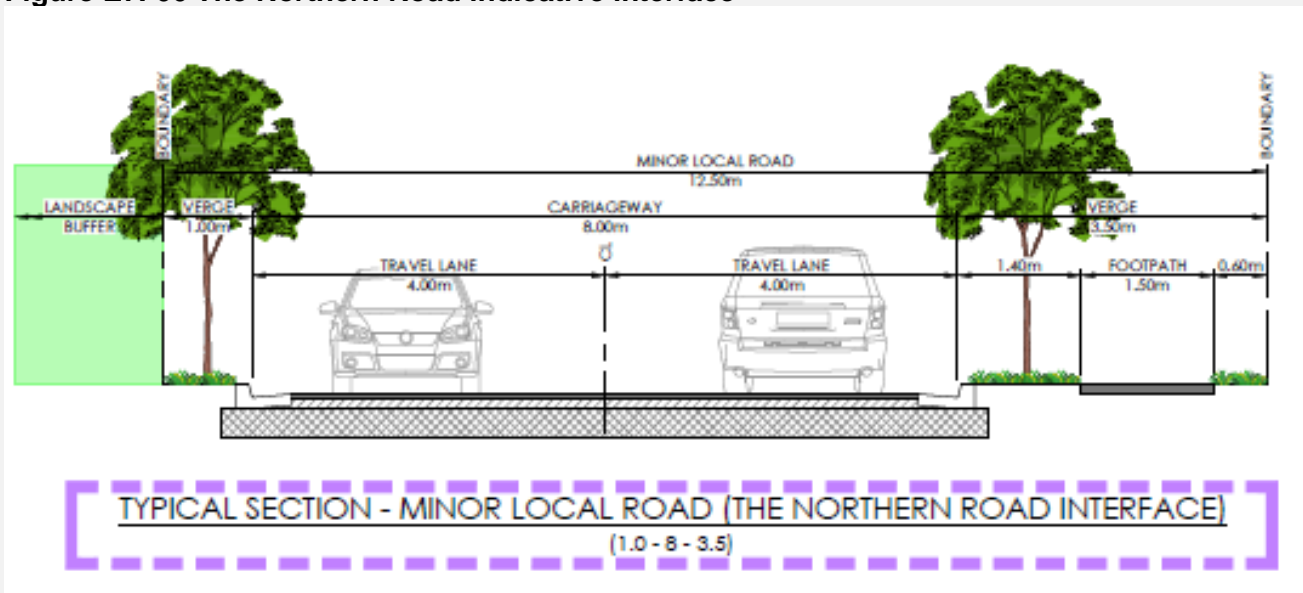
Figure E7. 66 The Northern Road indicative interface
