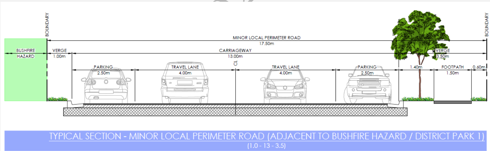
Figure E7.76-77 Minor Local Perimeter Road (Adjacent to Bushfire Hazard / District Park 1 & 2)
