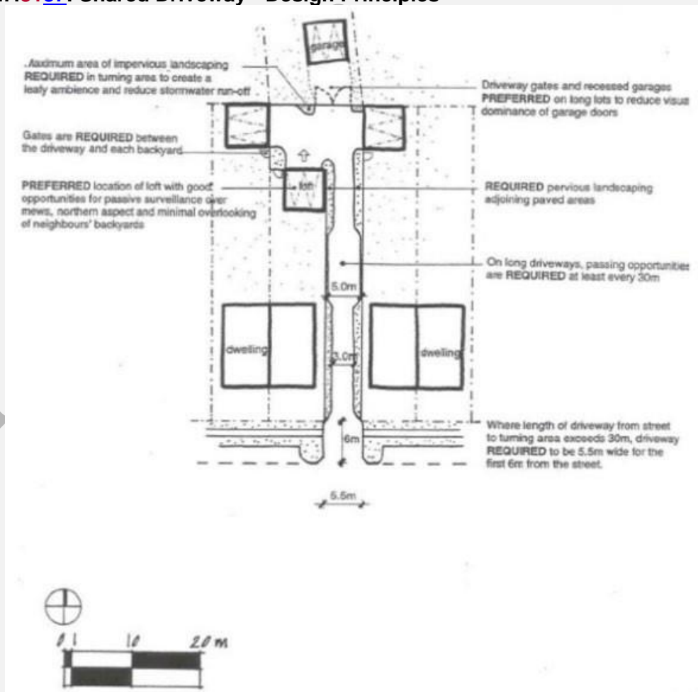
Figure E7.8187: Shared Driveway - Design Principles
