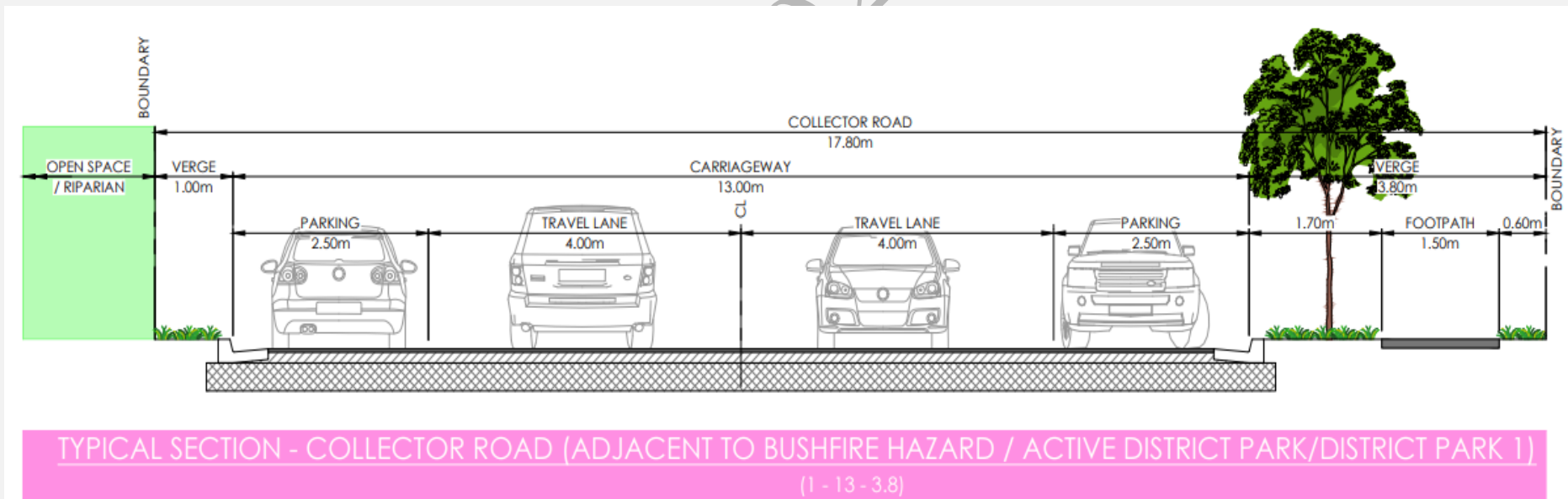
Figure E7.71 Collector Road (Adjacent to bushfire hazard / Active District Park/District Park 1 Open Space )
