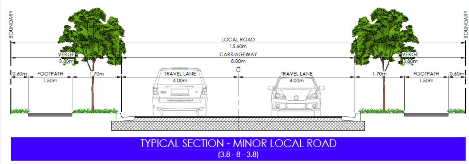
Figure E7.73-74 Minor Local Road
