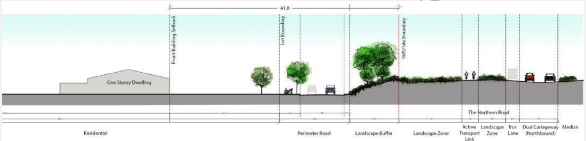
Figure E7.86-92 Cross Section of Lots fronting The Northern Road, Internal Perimeter Road and The Northern Road road reserve.
