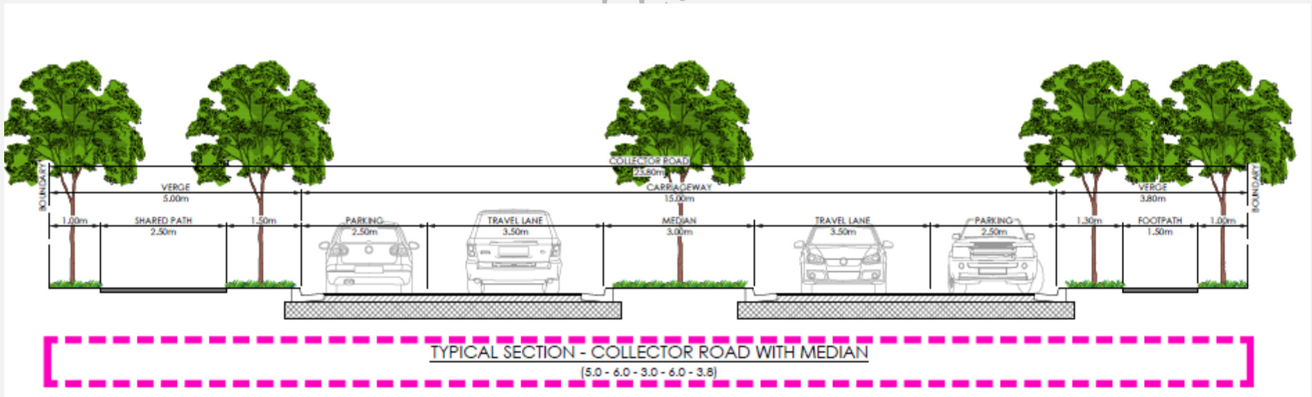
Figure E7.69 Collector Road with Median
