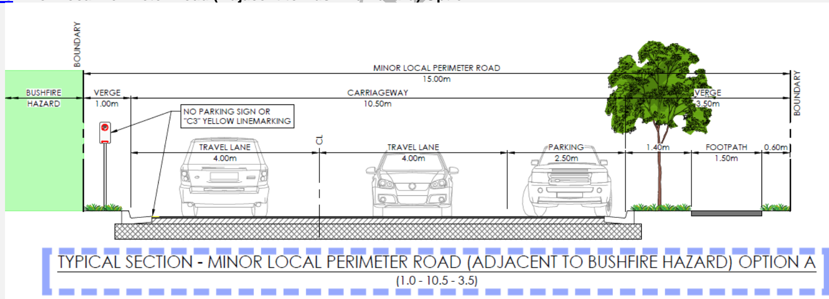
Figure E7.74-75 Minor Local Perimeter Road (Adjacent to Bushfire Hazard) Option A
