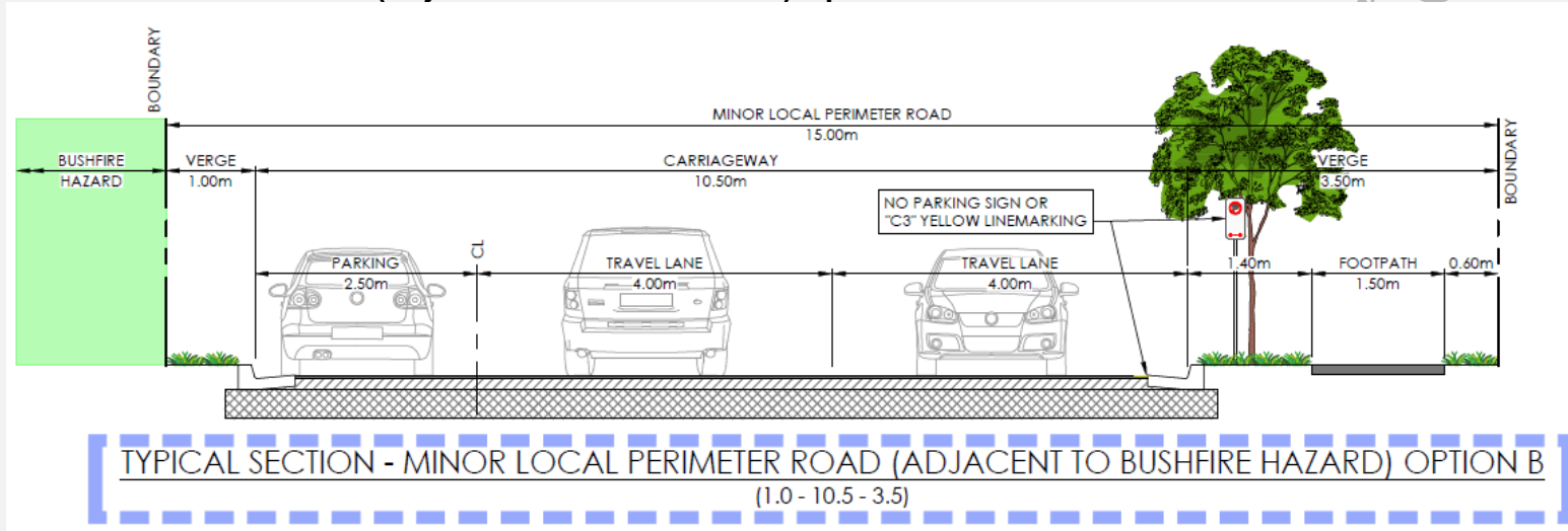
Figure E7.75-76 Minor Local Perimeter Road (Adjacent to Bushfire Hazard) Option B
