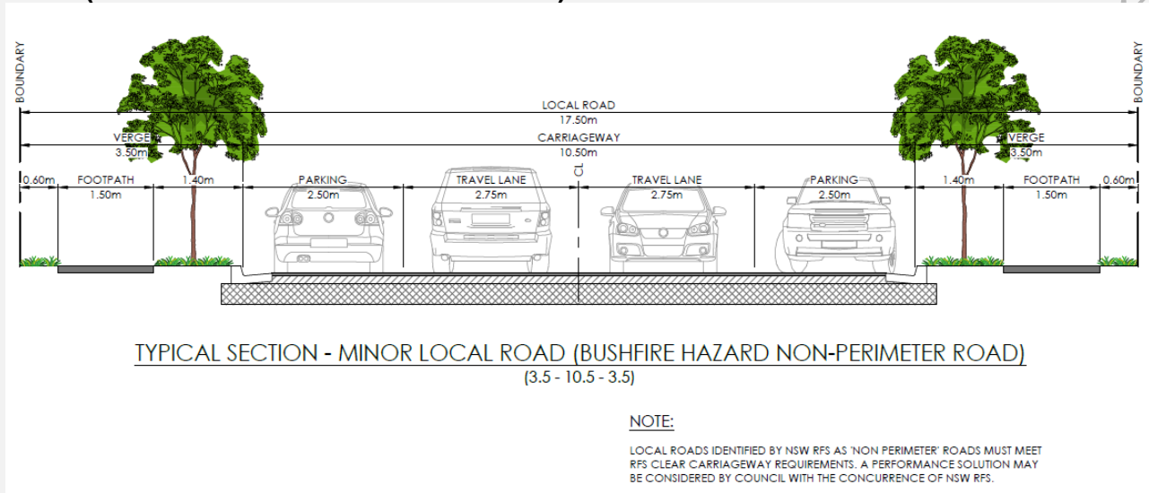
Figure E7.77-78 Minor Local Road (Bushfire Hazard Non-Perimeter Road)
