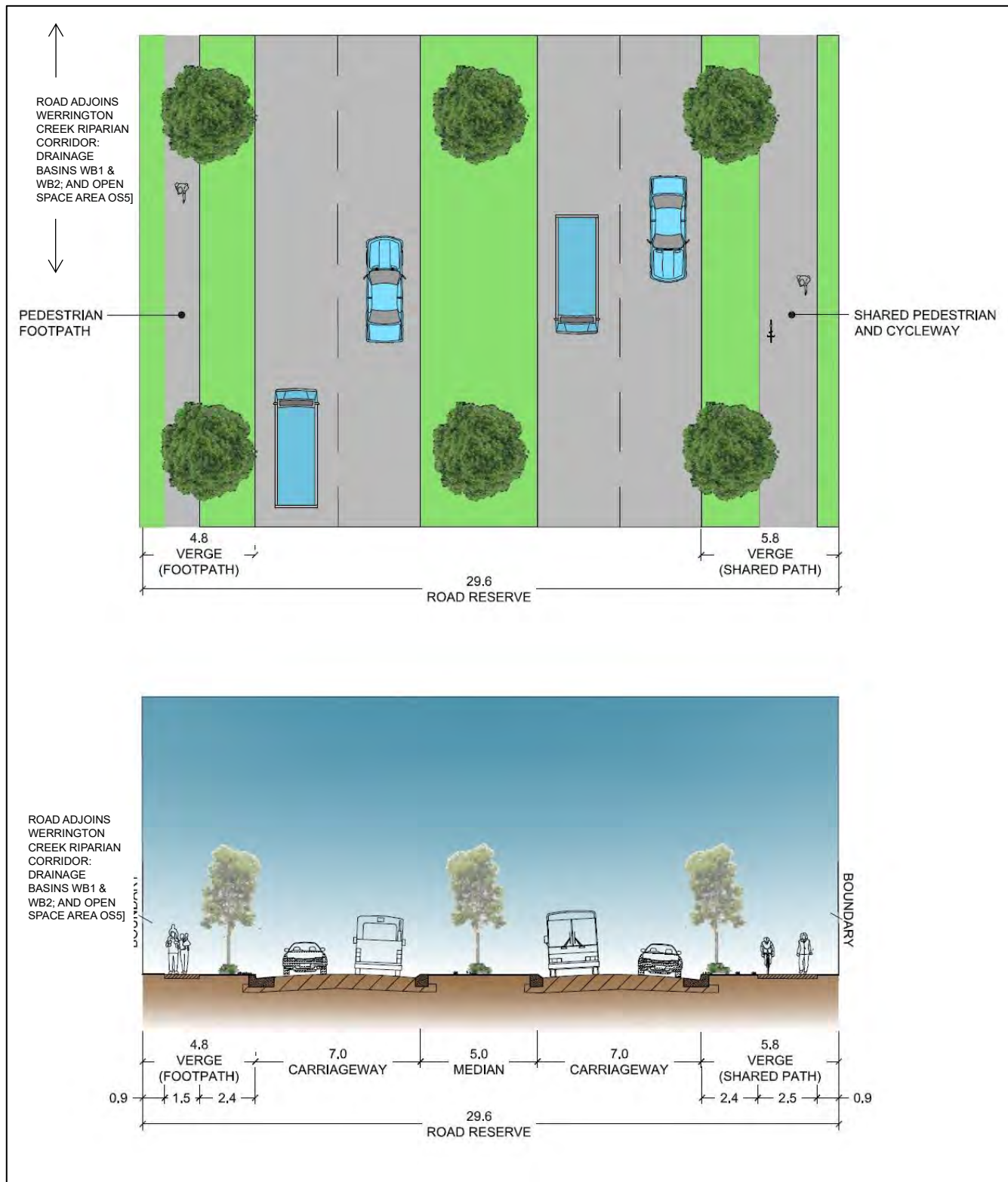
Figure E17.8: Typical street cross section – East-West Road (Western Section)
