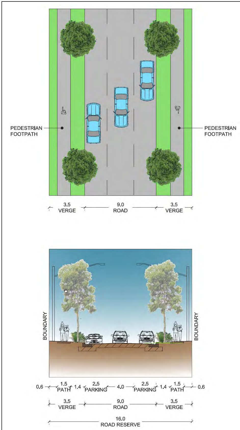
Figure E17.11: Typical street cross section – Minor Local Road
