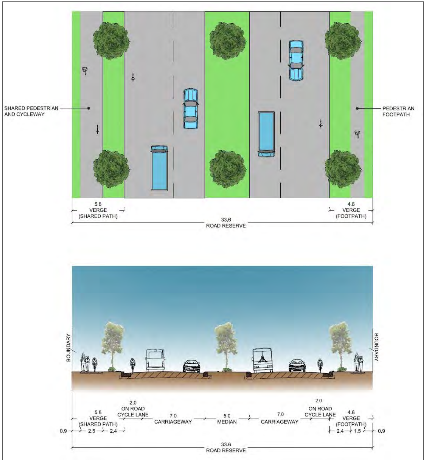
Figure E17.7: Typical street cross section – North-South Road
