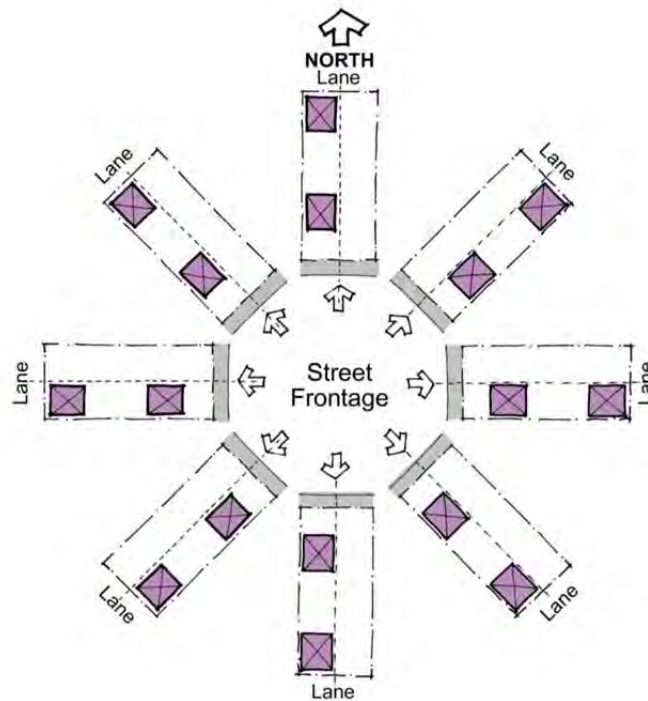
Figure E17.27: Garage Location Principles
