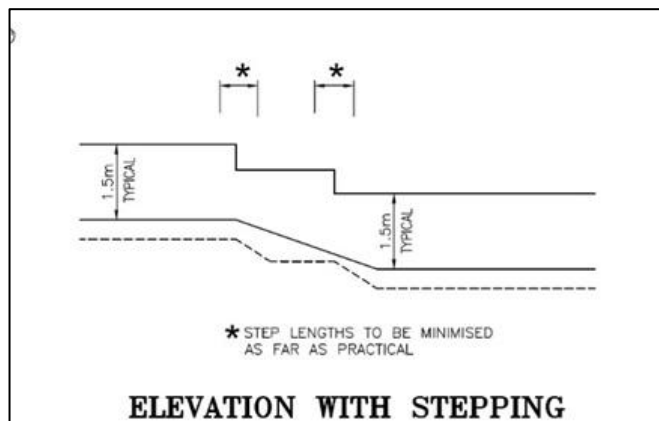
Figure E17.20: General Elevations
