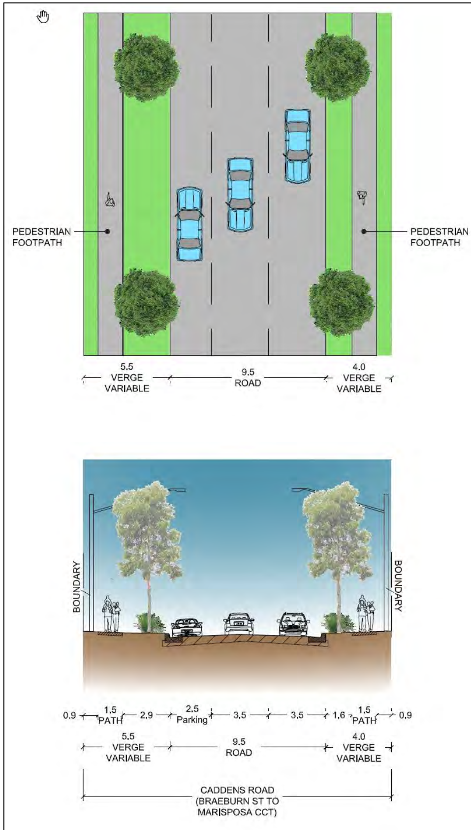
Figure E17.6: Typical street cross section – Caddens Road
