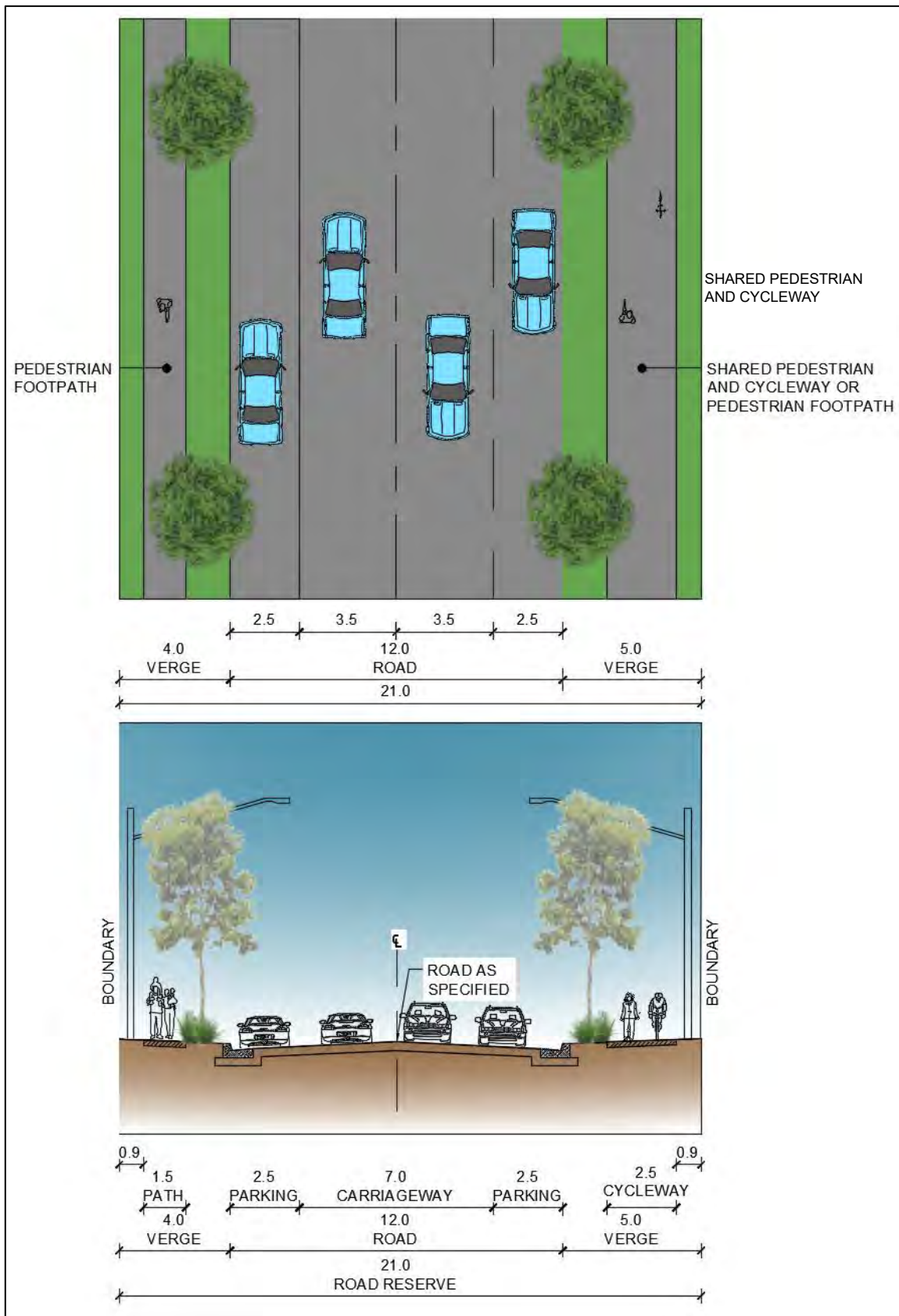
Figure E17.10: Typical street cross section – Major Local Road
