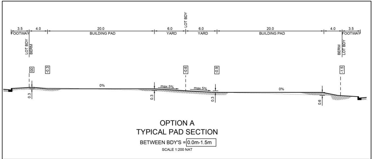
Figure E17.19: Typical Grading Solutions
