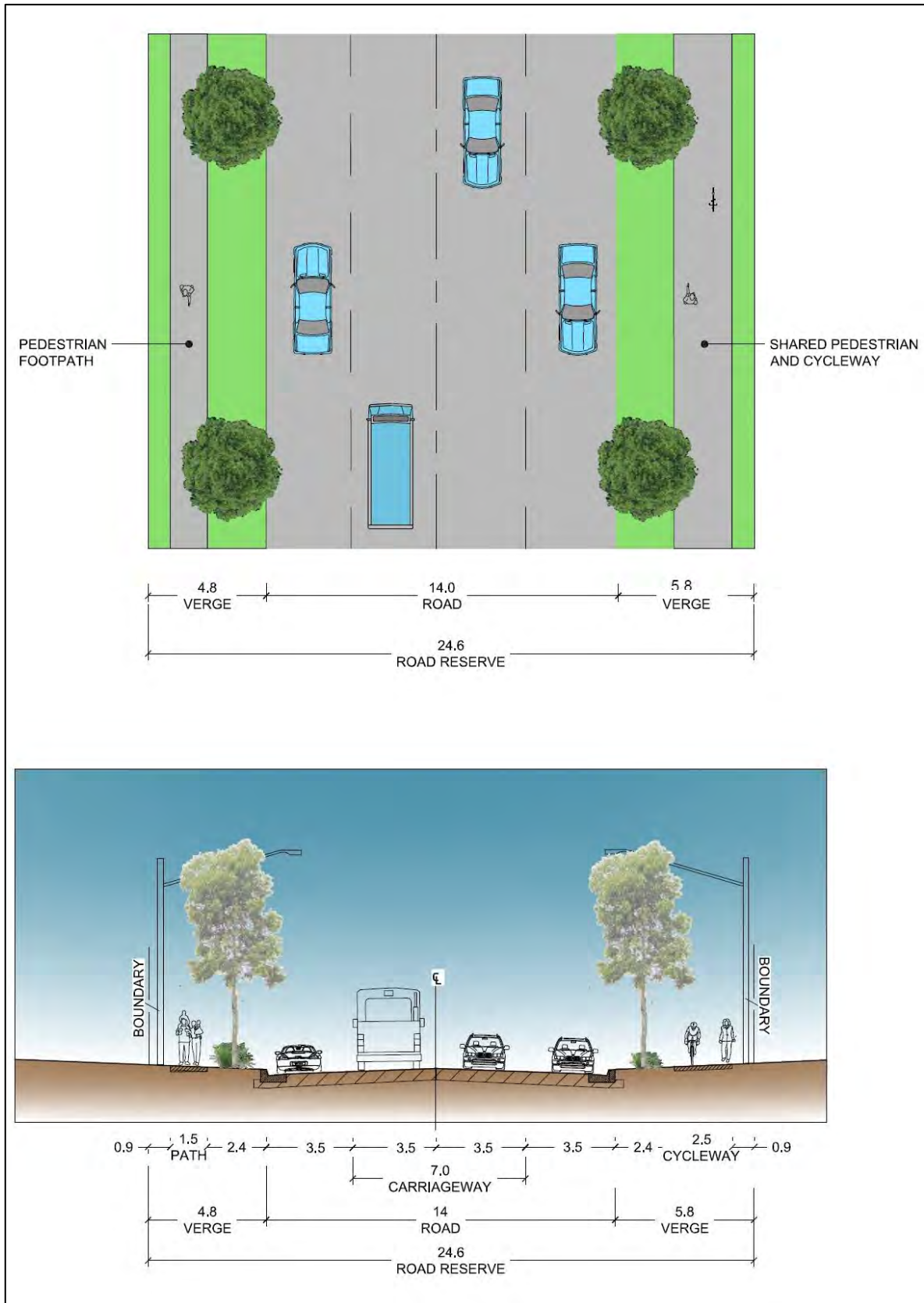
Figure E17.9: Typical street cross section – East-West Road (Eastern Section)
