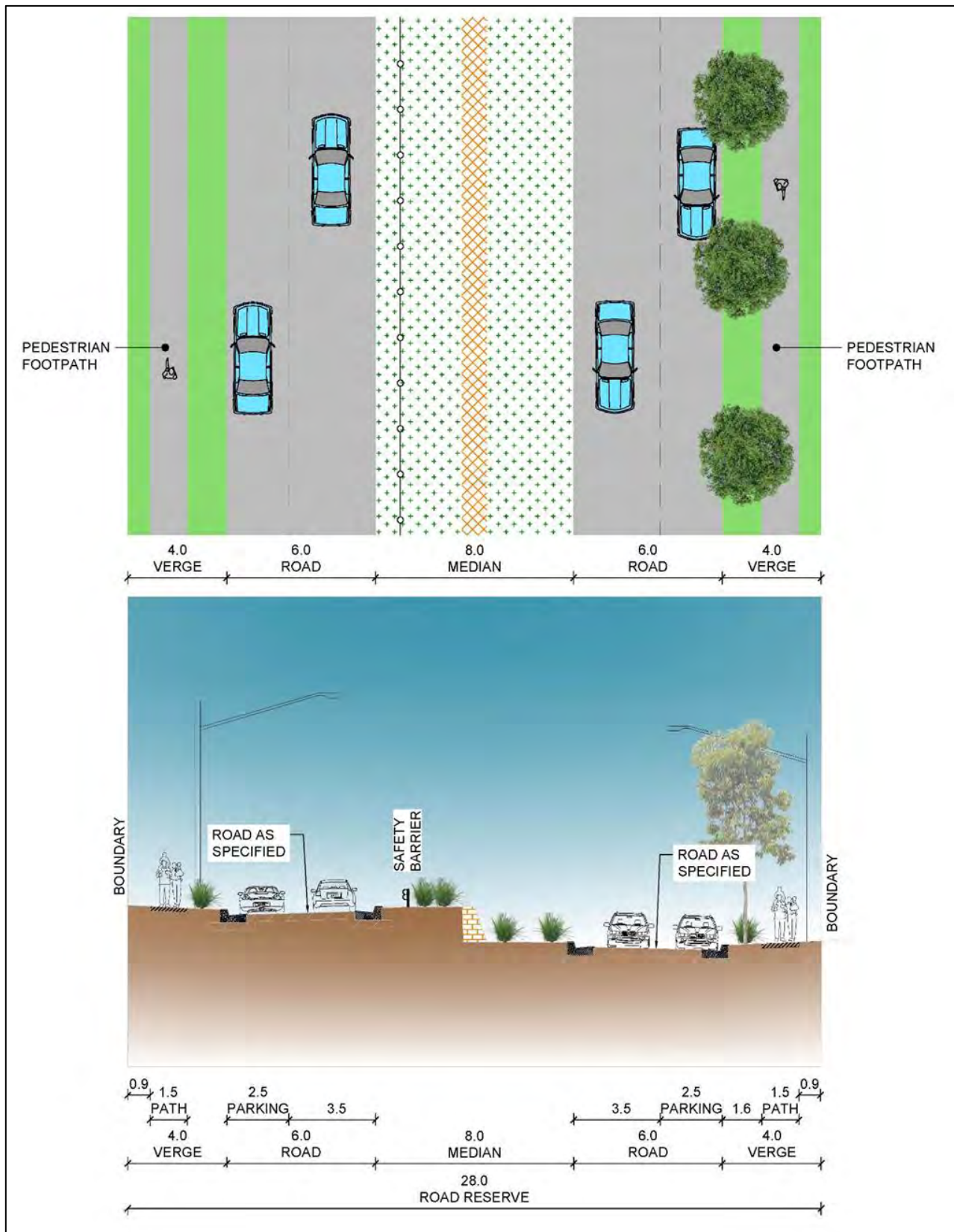
Figure E17.5: Typical street cross section - Split-level road
